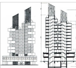
16. Kishō Kurokawa / Nakagin capsule tower, Tokyo, Japan, 1970-1972
