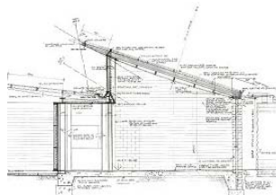
25. Glen Murcutt / House in the Adelaide Hills, Australia, 1998
