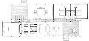
19. Glenn Murcutt / Marie Short house, 1974-75
