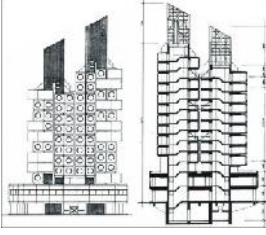
17. Kish Kurokawa / Nakagin capsule tower, Tokyo, Japan, 1970-1972
