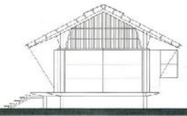
30. Glenn Murcutt / Marika House, Yirrkala Community, Eastern Arnhem Land, Australia, 1994
